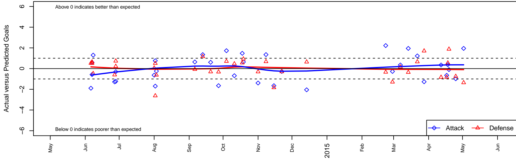
WPFC Fury Black G01 Dots are actual minus expected GF (blue circles) and GA (red triangles). Blue line is smoothed change in attack strength. Red is smoothed change in defense strength.
